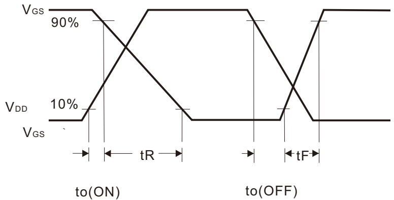
Switching Waveforms
