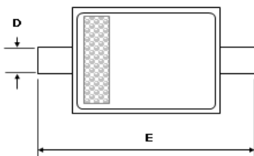
SOD323F * Package Outline
