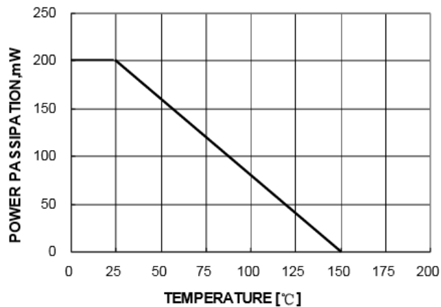
POWER DISSIPATION VS. AMBIENT TEMP
