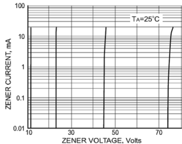
ZENER BREAKDOWN CHARACTERISTICS
